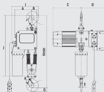
ECJ4 · 2,000 Kg. (schematic only)
