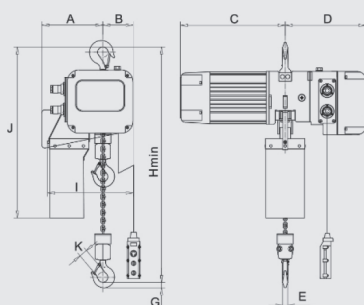
ECJ4 · 500 kg - 1,000 kg (schematic only)
