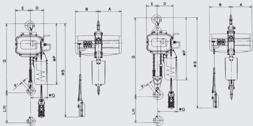
ECH4 · 500 Kg - 1.000 Kg (schematic only)
