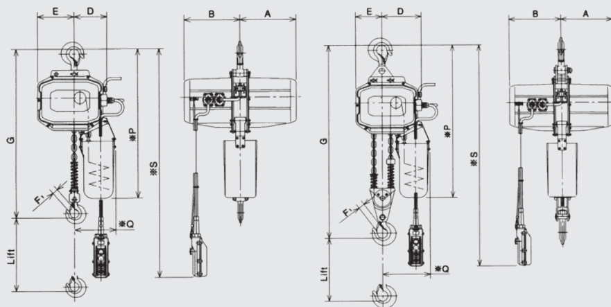
ECCH4 · 500 Kg - 1000 Kg. (schematic only)
